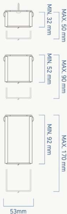
Height Adjustment Bracket
