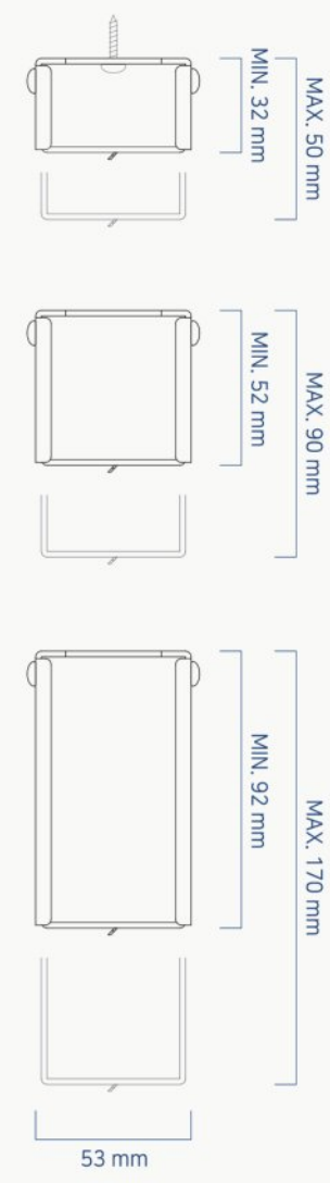
Height Adjustment Bracket
