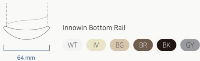
Bottom Rail Info for Innowin Shades (Single model)
