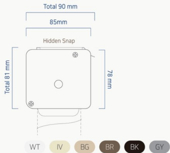
Bottom Rail Info for Innowin Shades (Single model)
